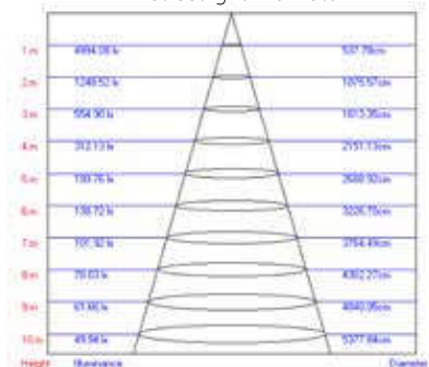
LED Streetlight 140 Watt
